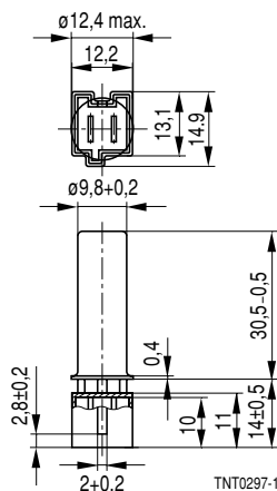
Dimensions in mm Approx. weight 10 g
